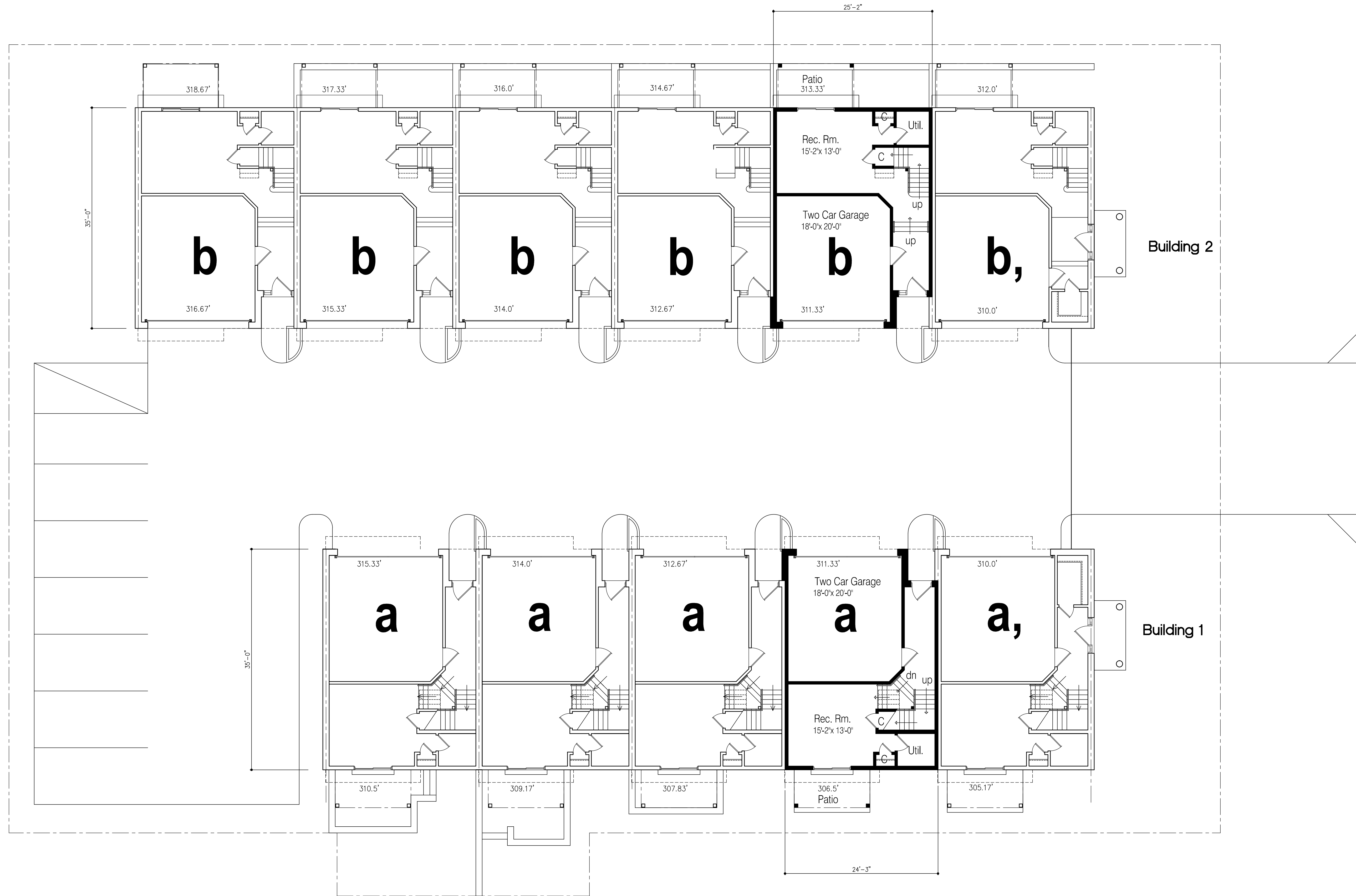
Ground Floor Plan 1/8" = 1'-0"
